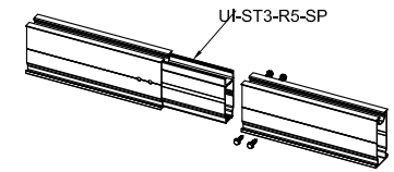
Rail Splice
